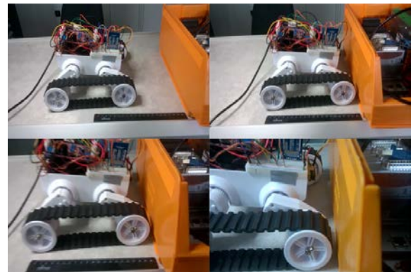
Fig. 6. Test of collision avoidance
