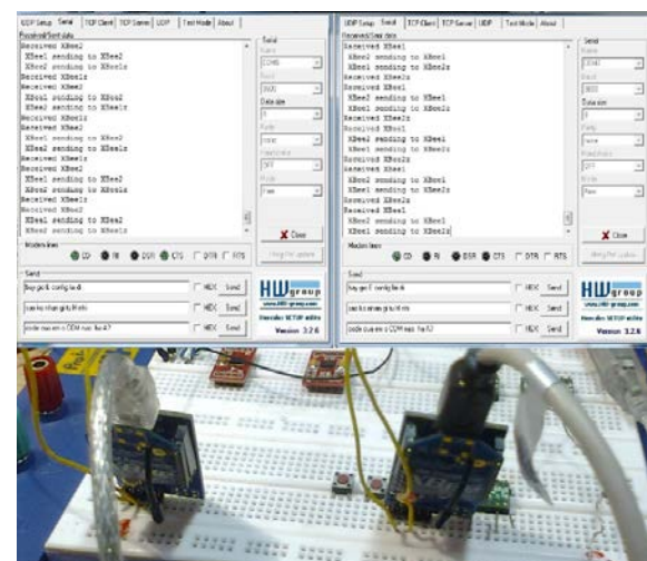
Fig. 10. Communication among XBees
