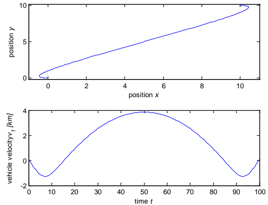
Fig. 5. Feasible path and velocity solution
