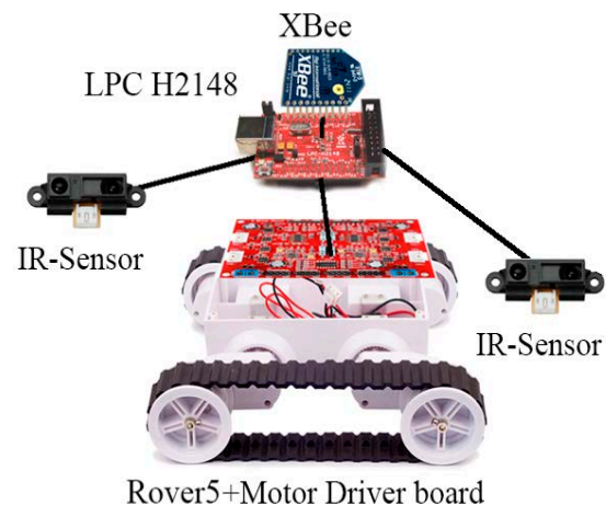
Fig. 1. Mobile robots configuration
